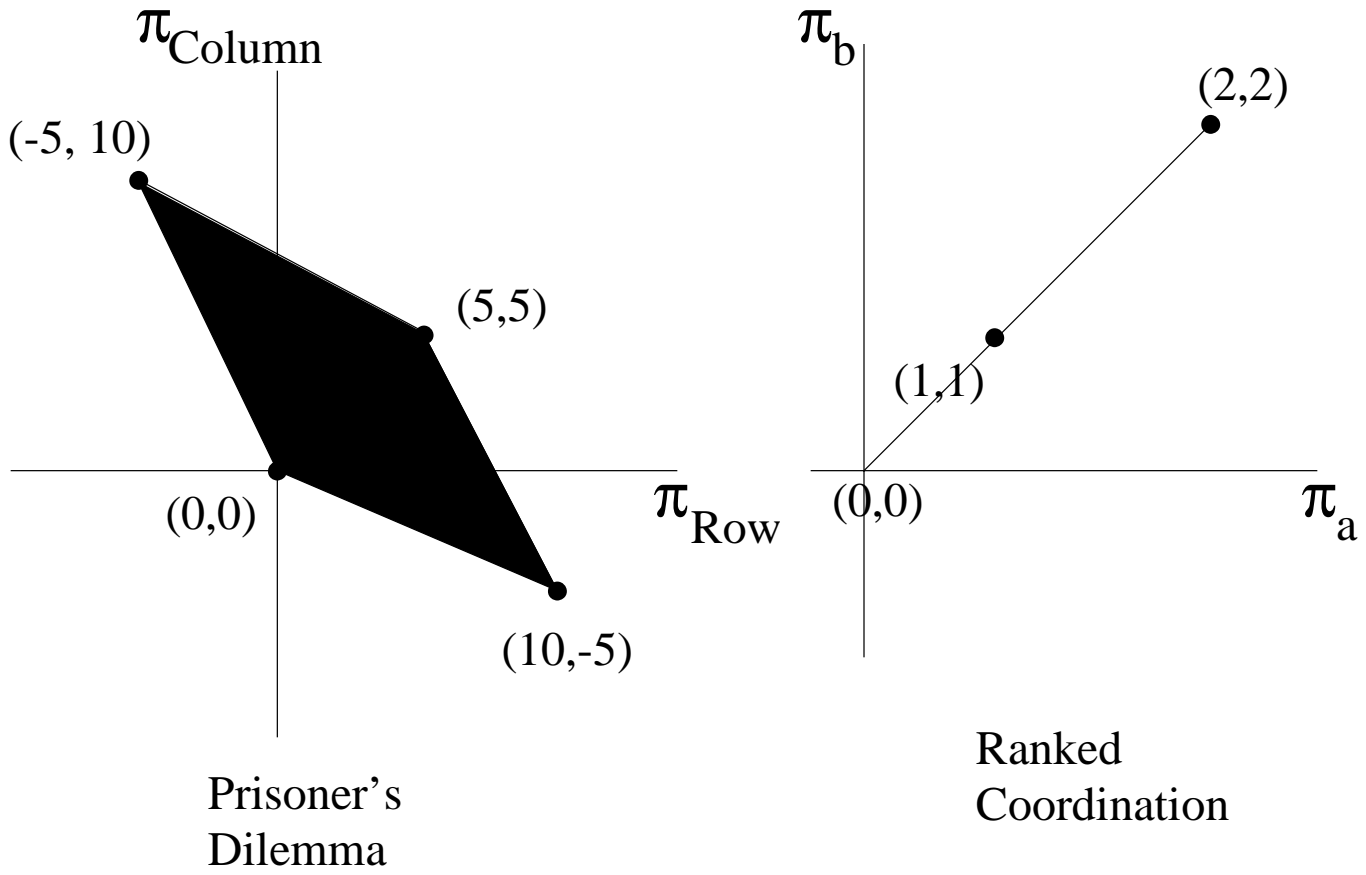
Figure 5.1 The Dimensionality Condition
