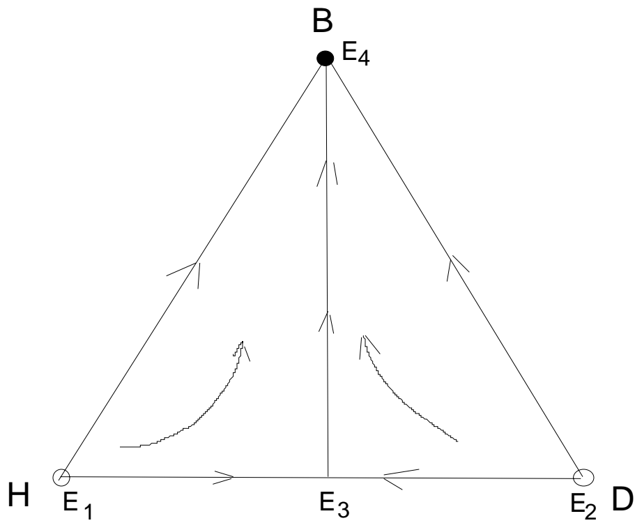
Figure 4.7 Evolutionary Dynamics in “The Hawk-Dove-Bourgeois Game”
