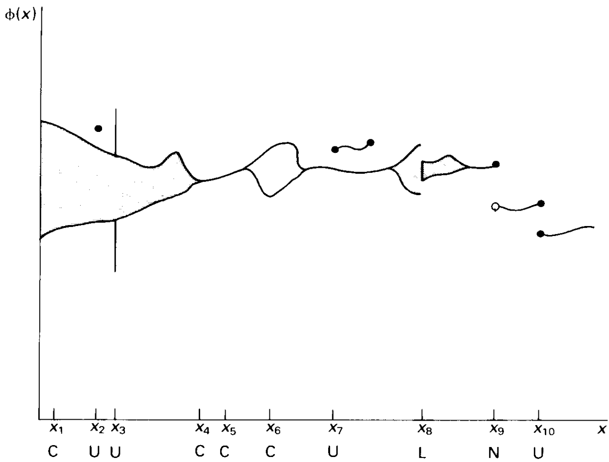
Figure A.2 Upper semicontinuity
